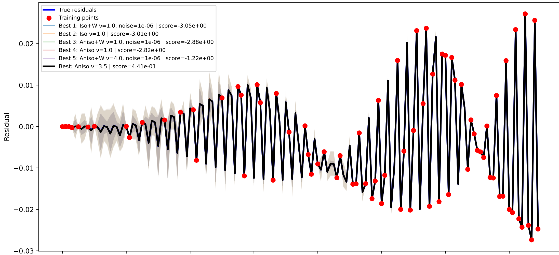
GPR kernel comparison node=47 RMSE=1.903e-05, train RMSE=5.801e-11
